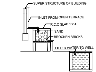
DETAILS OF FILTER BED & WELL
