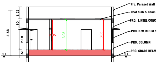
CROSS SECTION ON AB
