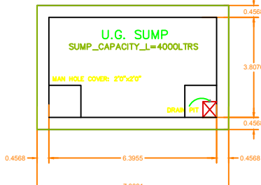
SUMP DETAIL
