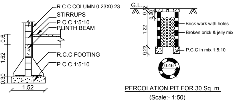
COLOUMN DETAILS
