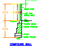
COMPOUND WALL DETAIL
