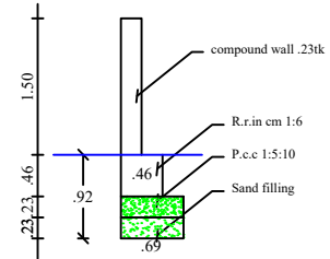
Compound wall Detail
