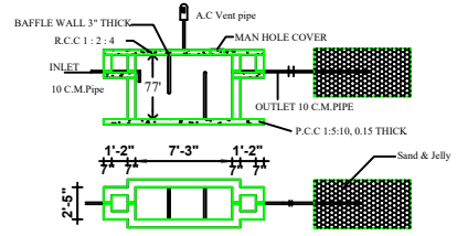
Septic tank and trench
