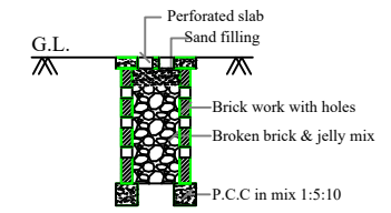
PERCOLATION PIT FOR 30 Sq. m. (NOT FOR SCALE)
