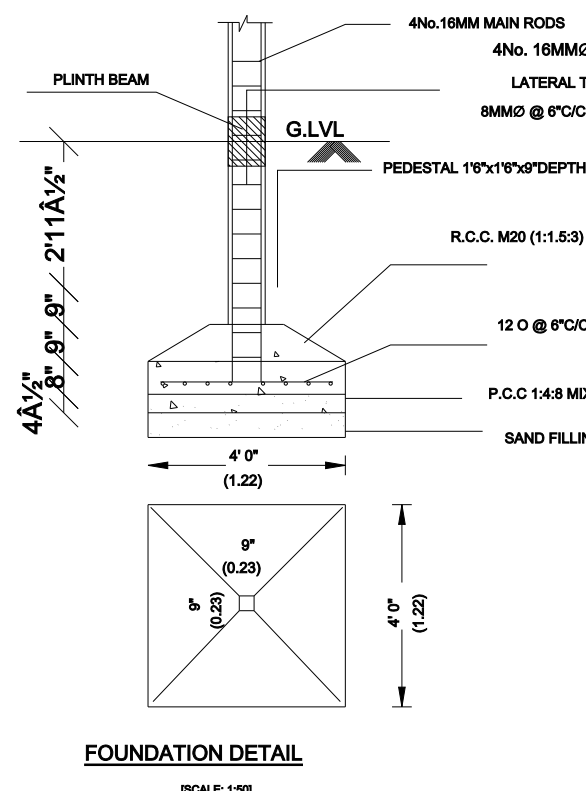
FOUNDATION DETAILS
