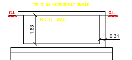
RWHS SECTION (SAMPLE) RWHS_CAPACITY_L = 2000LTRS
