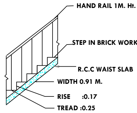
STAIR DETAIL
