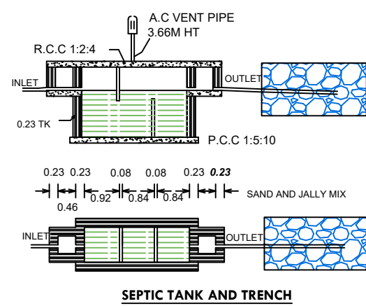
SEPTIC TANK AND TRENCH
