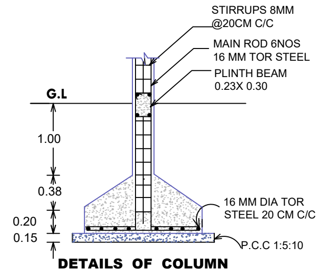
DETAILS OF COLUMN
