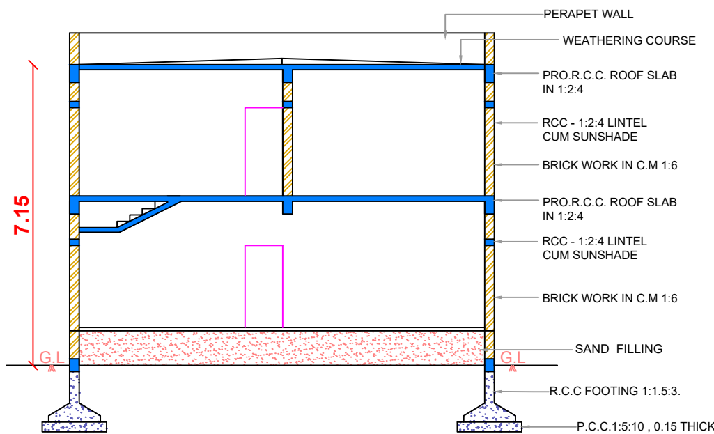
SECTION AB
