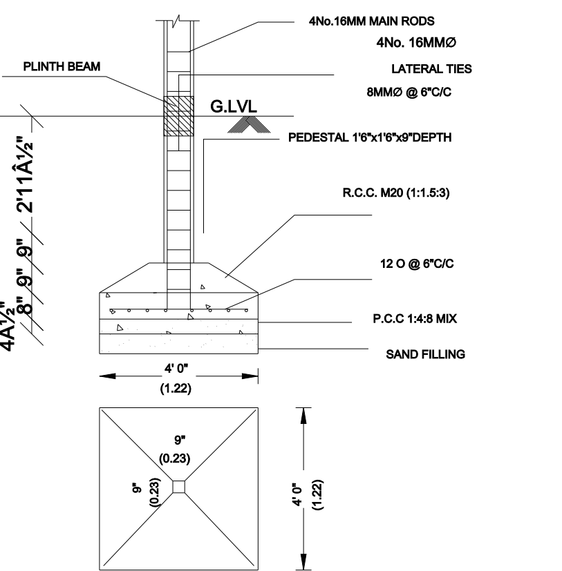
FOUNDATION DETAIL
