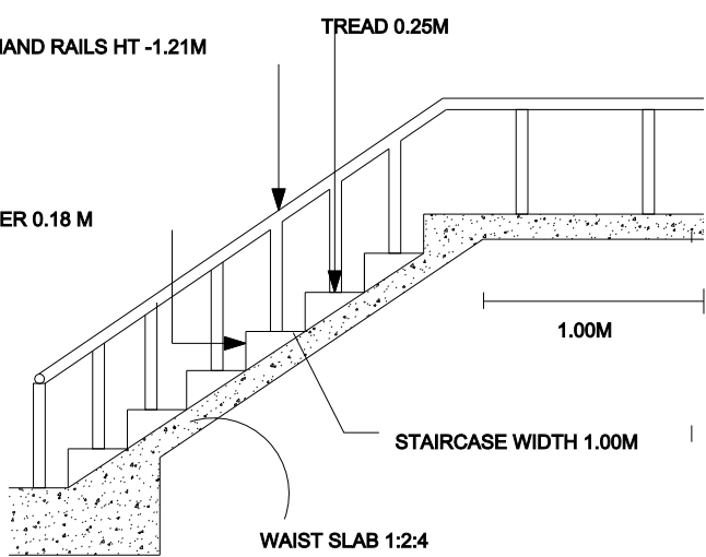
STAIRCASE DETAILS
