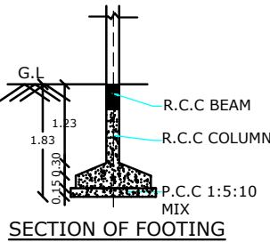
SECTION OF FOOTING
