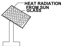
SOLAR SYSTEM
