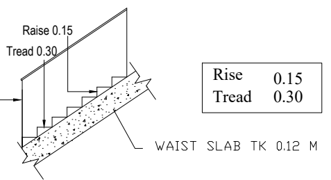
STAIRCASE DETAIL
