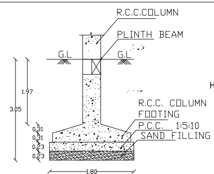
FOUNDATION DETAIL
