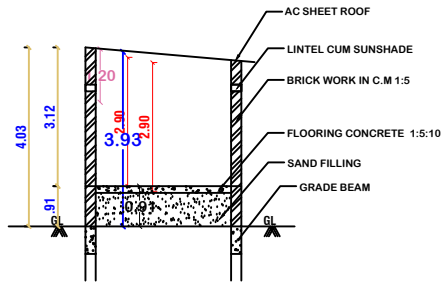
SECTION-AB
