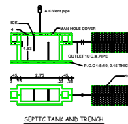
SEPTIC TANK AND TRENCH
