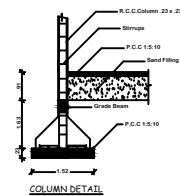
COLUMN DETAIL
