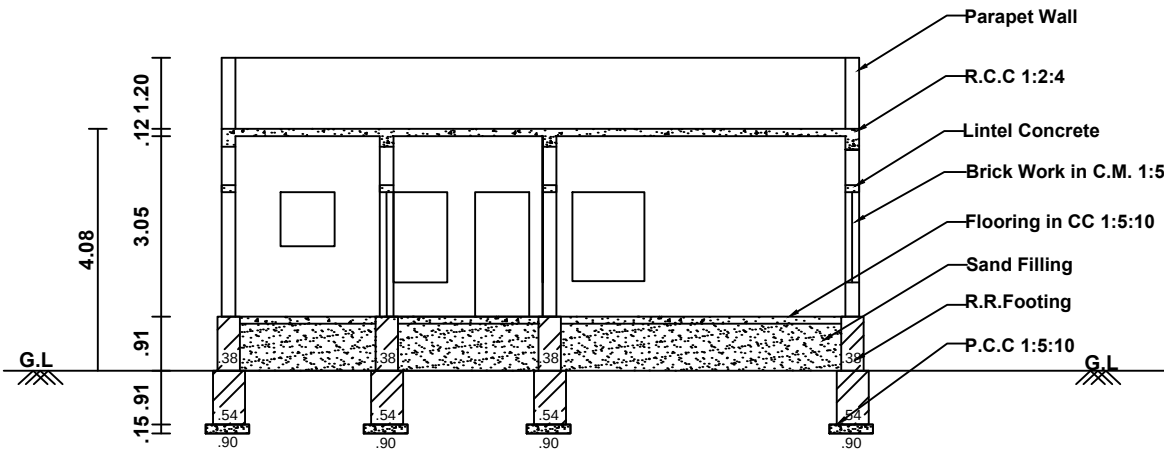
SECTION "AB"
