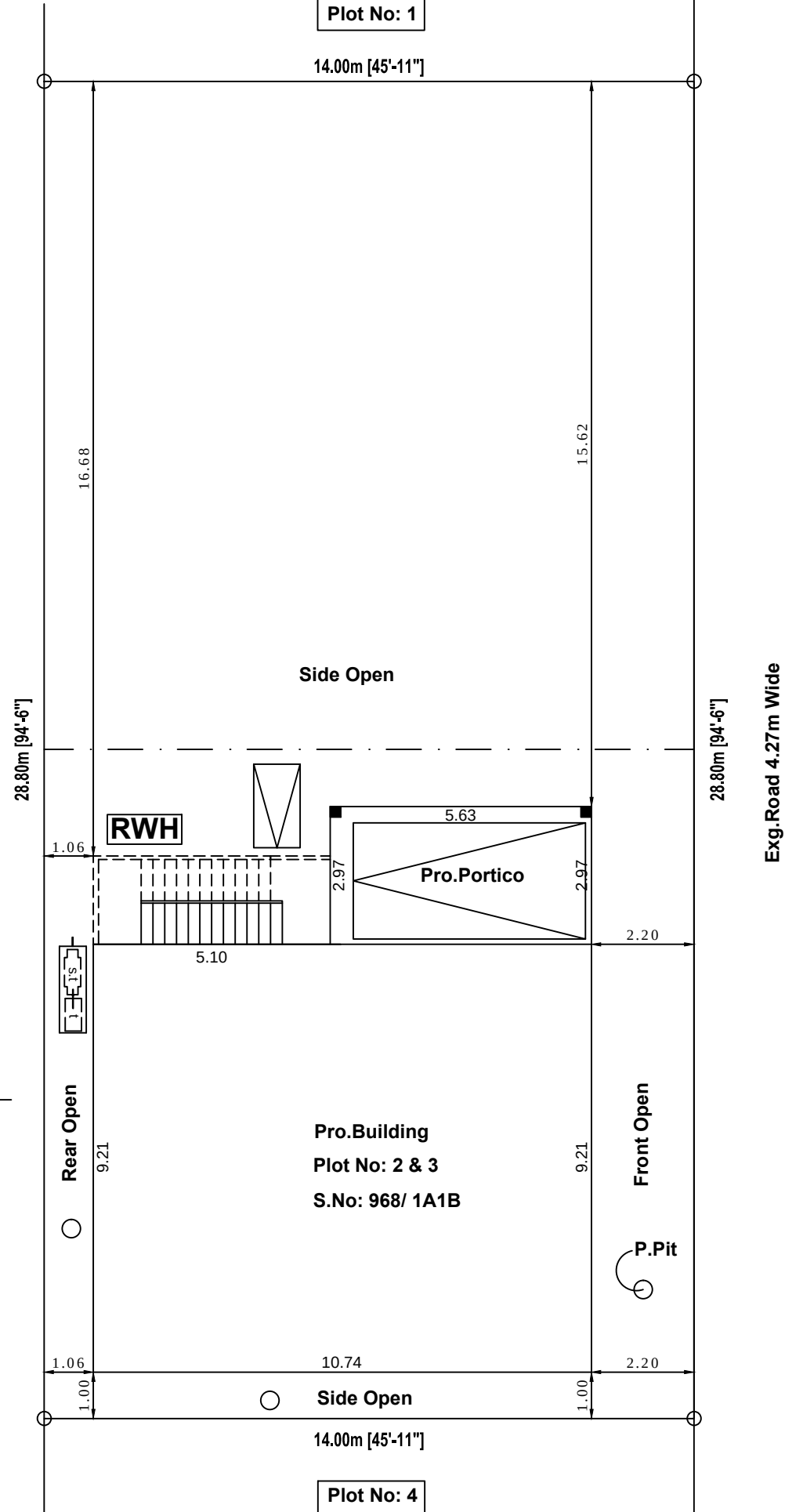
SITE PLAN
