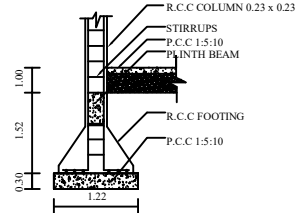
COLUMN DETAILS
