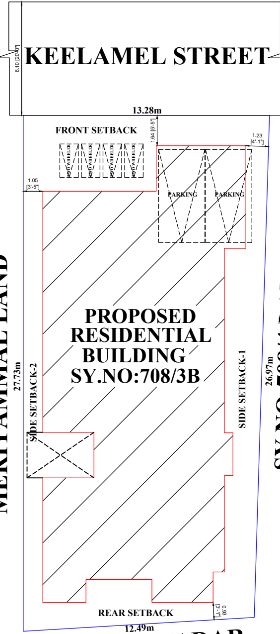
THARSIS NADAR VAGAIYARA LAND SITE PLAN(SCALE 1:100)
