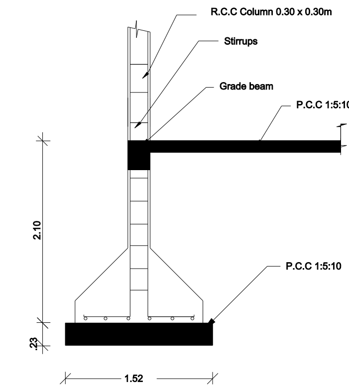
Column Detail
