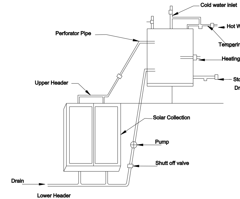
Details Of Solar Water Heater (NTS)
