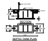
SEPTIC TANK (Scale 1:100)
