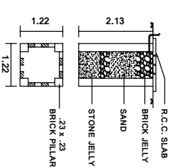
PLAN & SECTION OF RAIN WATER COLLECTION WELL
