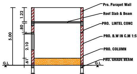
CROSS SECTION ON AB
