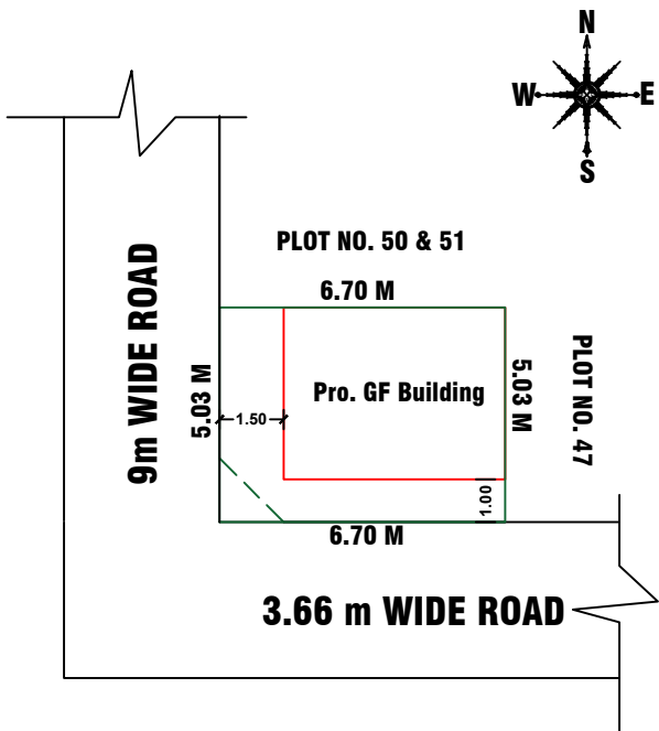
SITE PLAN
