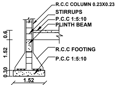
COLOUMN DETAILS
