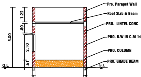
CROSS SECTION ON AB
