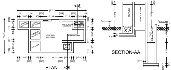
SEWAGE TREATMENT PLANT (NOT TO SCALE)
