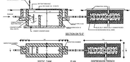
TYPE DESIGN FOR A SEPTIC TANK 10,000 Lts CAPACITY (NOT TO SCALE)
