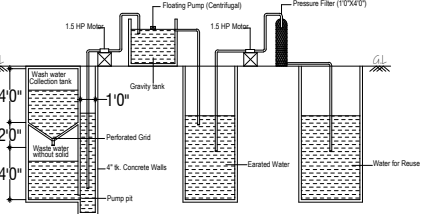
WASTE WATER RECYCLE PLANT DETAILS (NOT TO SCALE)
