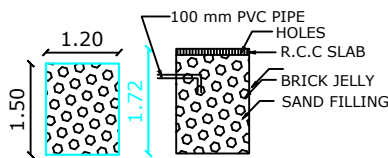
PLAN & SECTION OF RAIN WATER COLLECTION TANK
