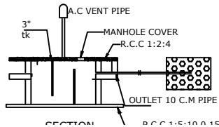
PLAN & SECTION OF RAIN WATER COLLECTION TANK
