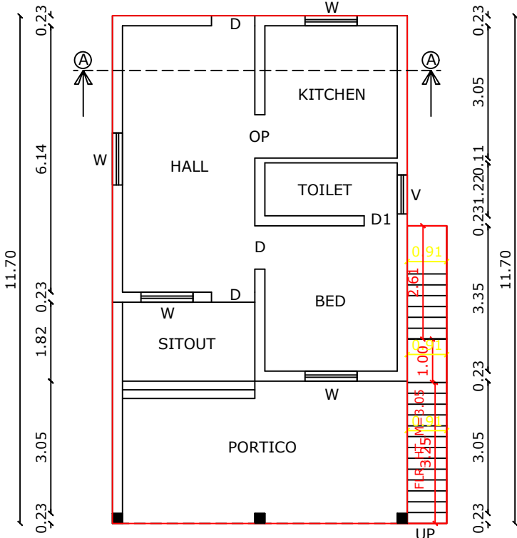
GROUND FLOOR PLAN (EXISTING)
