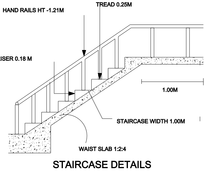
STAIRCASE DETAILS
