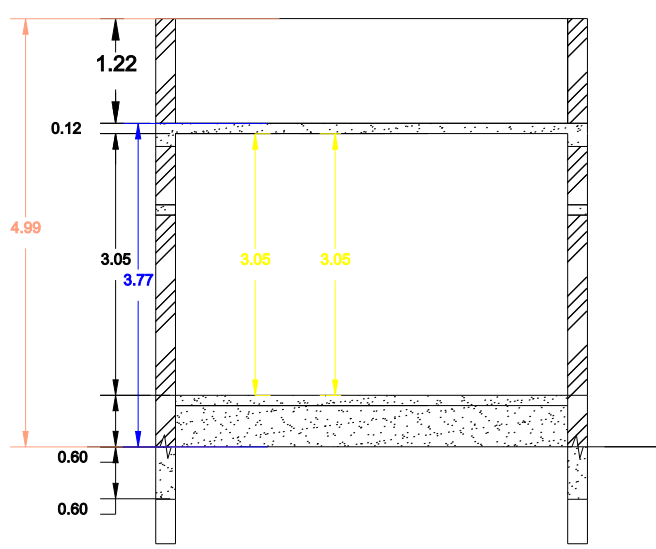
SECTION - "AB"
