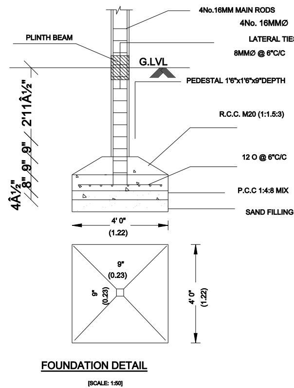
FOUNDATION DETAIL
