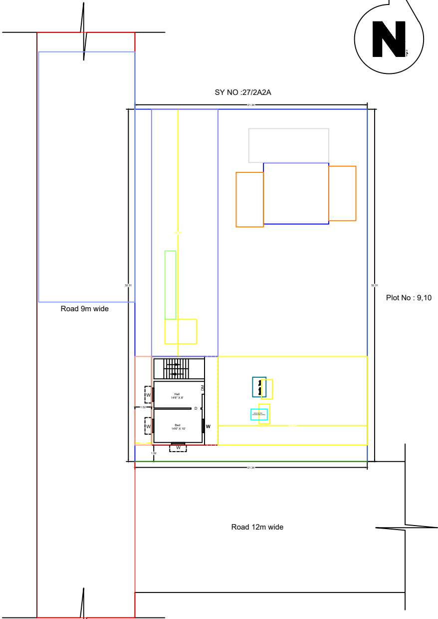
SITE PLAN
