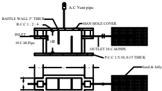
SEPTIC TANK AND TRENCH
