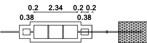
PLAN OF SEPTIC TANK & TRENCH
