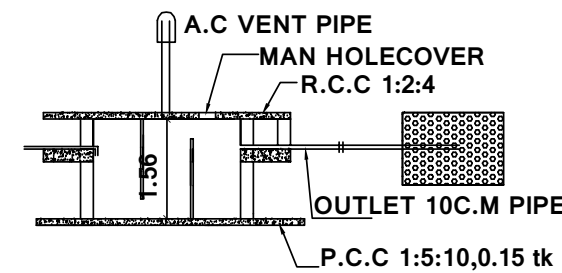
SECTION
