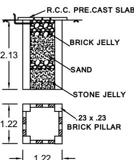
PLAN & SECTION OF RAIN WATER COLLECTION WELL
