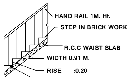
STAIR DETAIL
