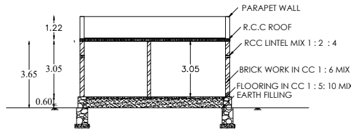
SECTION ON AB & ( HALF ELEVATION )
