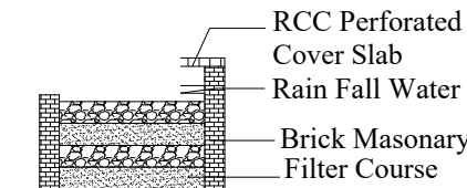
PLAN SECTION OF RECHARGE TRENCH METHOD
