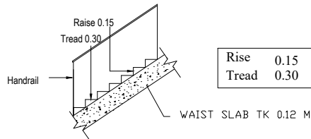
STAIRCASE DETAIL
