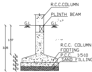
FOUNDATION DETAIL
