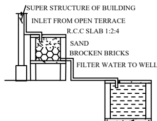
Rainwater harvesting
