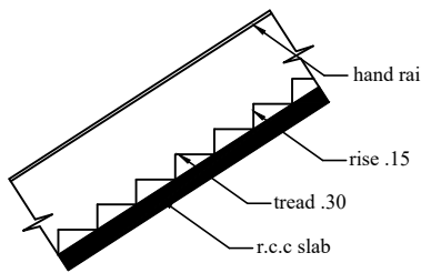
STAIR
