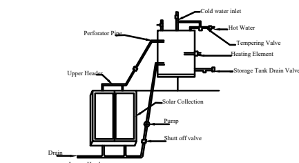
details of Solar Water Heater (NTS)
