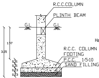
FOUNDATION DETAIL
