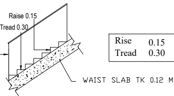
STAIRCASE DETAIL
