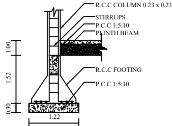
COLUMN DETAILS
