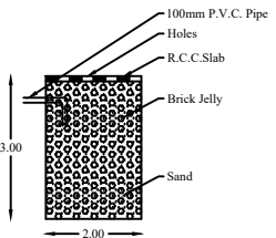
SECTION OF RAIN WATER COLLECTING TANK
