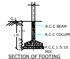
SECTION OF FOOTING
