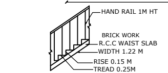
STAIRCASE DETAIL
