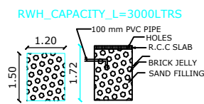
PLAN & SECTION OF RAIN WATER COLLECTION TANK
