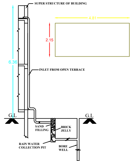
RAIN WATER HARVESTING SYSTEM RWH_CAPACITY_L=1000LTRS
