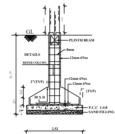
FOUNDATION DETAILS SCALE : 1:50
