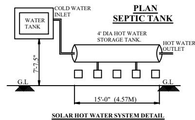
SOLAR HOT WATER SYSTEM DETAIL
