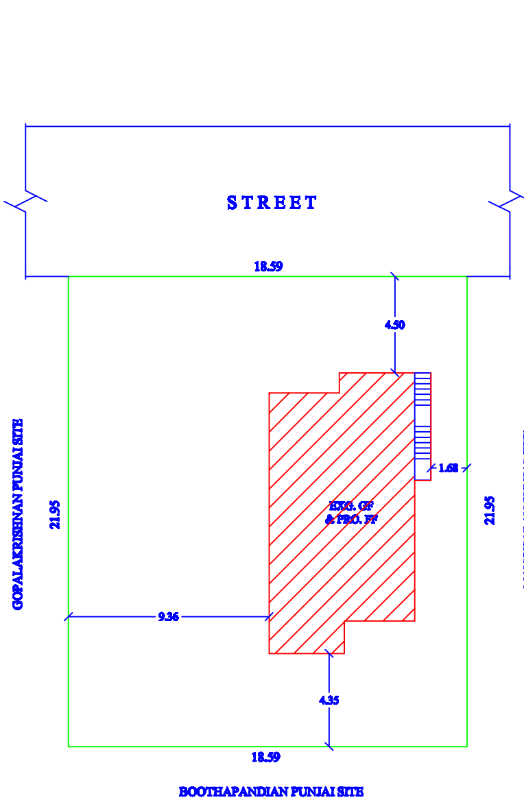
TOPO PLAN
