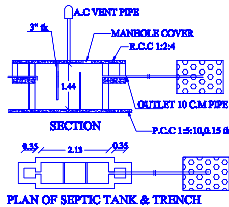
PLAN OF SEPTIC TANK & TRENCH
