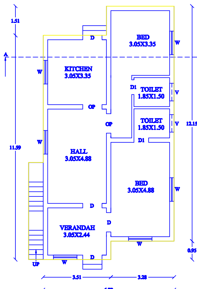
GROUND FLOOR PLAN (EXISTING)
