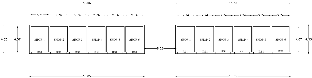
PRO BLOCK - 1 GROUND FLOOR PLAN
