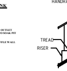
STAIRCASE DETAILS
