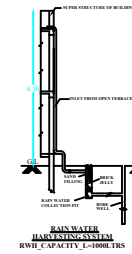
RAIN WATER HARVESTING SYSTEM
