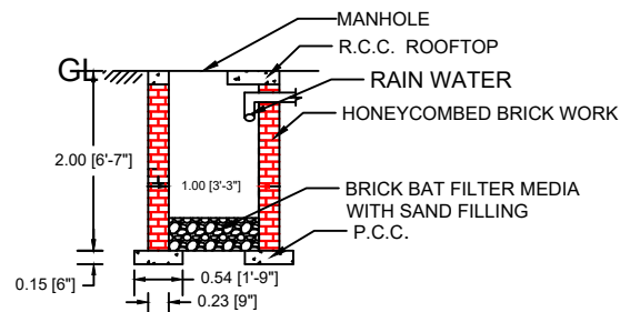
SECTION ON O - P
