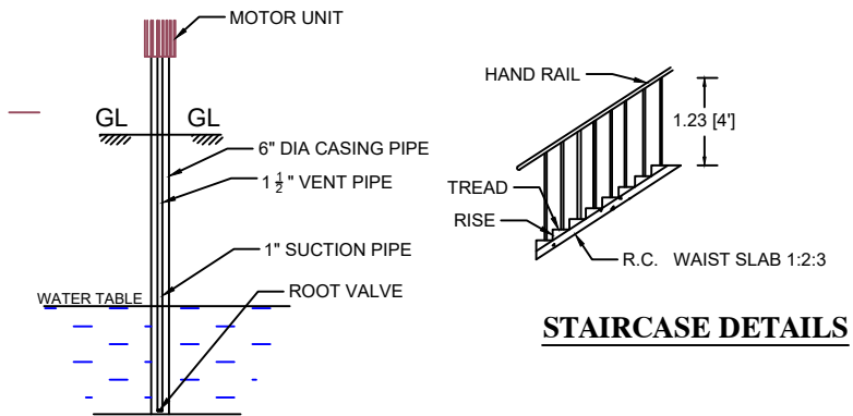
SEC.OF BOREWELL
