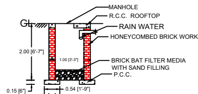
SECTION ON O - P
