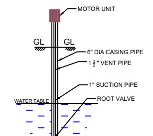
SEC.OF BOREWELL
