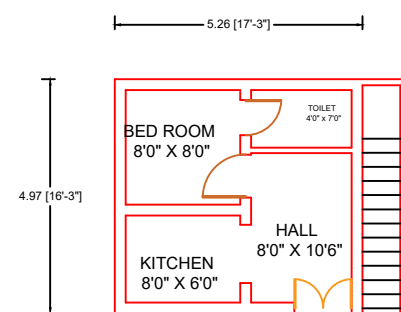
G.F. PLAN
