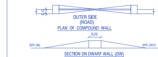
SECTION ON DWARF WALL (DW)
