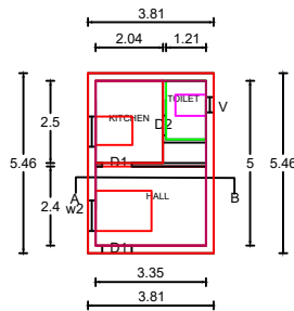
GROND FLOOR PLAN
