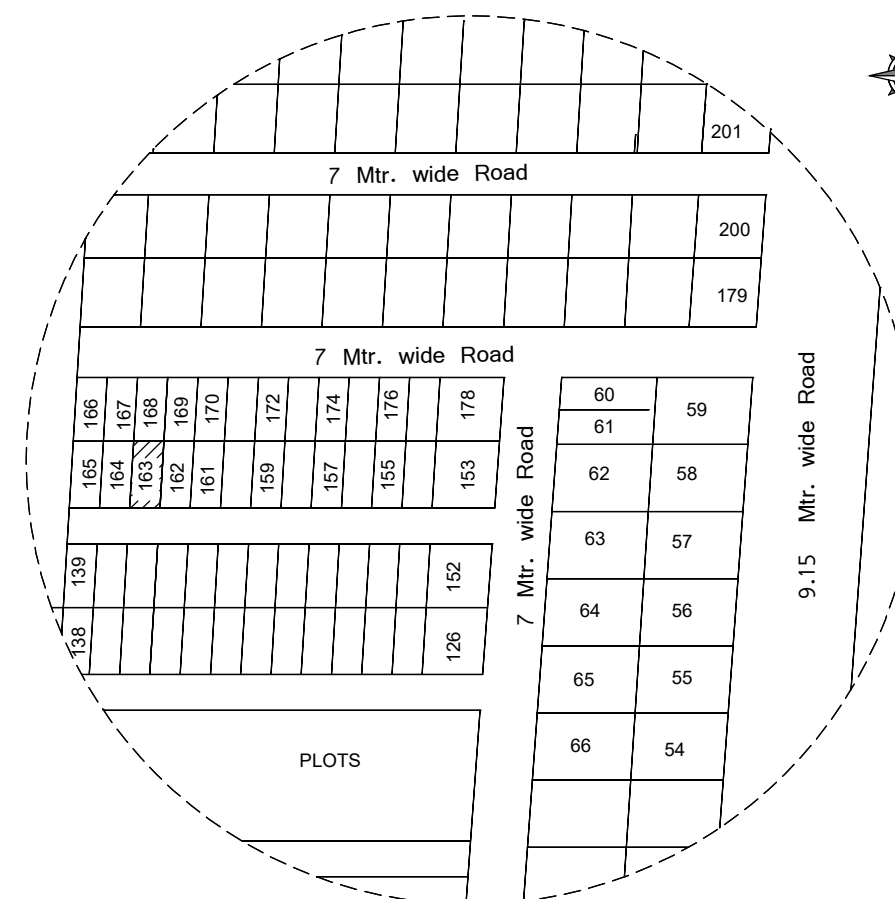
TOPO PLAN
