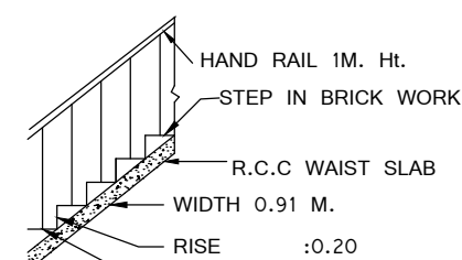
STAIR DETAIL
