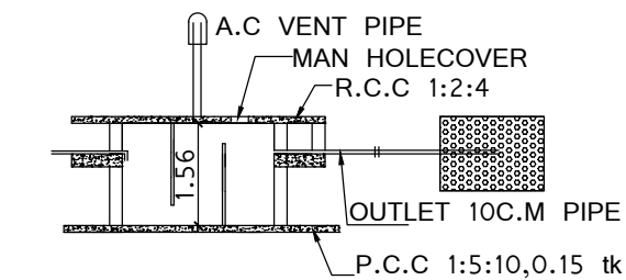
SECTION
