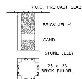
PLAN & SECTION OF RAIN WATER COLLECTION WELL
