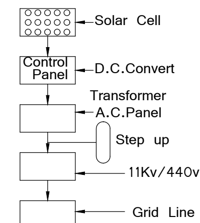
SOLAR SYSTEM
