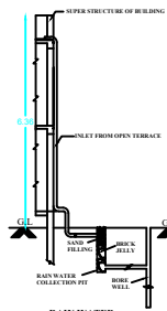
RAIN WATER HARVESTING SYSTEM RWHL CAPACITY L=1000LTRS
