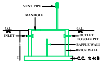
SECTION OF SEPTIC TANK
