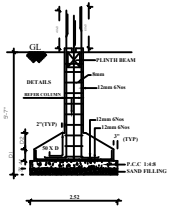
FOUNDATION DETAILS SCALE : 1:50
