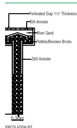
PERCOLATION PIT
