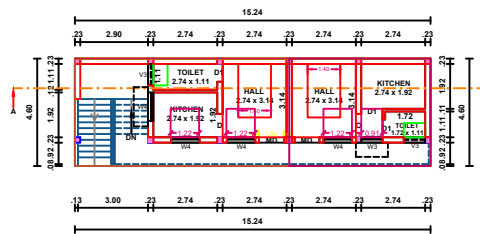
PRO. FIRST FLOOR
