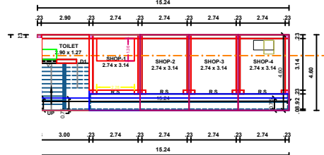
PRO. GROUND FLOOR
