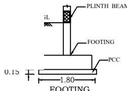
FOOTING
