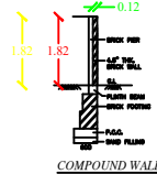
DETAIL
