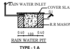
RAIN WATER PIT TYPE - 1 A
