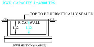
RWHS SECTION (SAMPLE)
