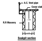
Soakpit section
