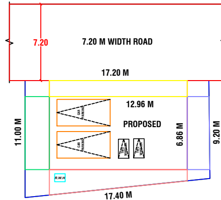
17.40 M SITE PLAN SCALE 1:100
