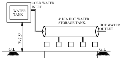
SOLAR HOT WATER SYSTEM DETAIL
