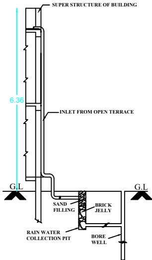
RAIN WATER HARVESTING SYSTEM RWH_CAPACITY_L=1000LTRS
