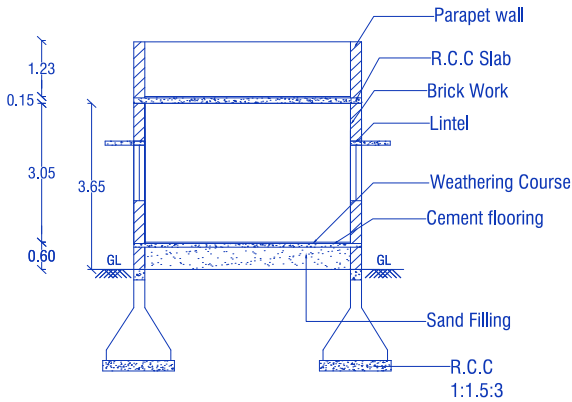
CROSS SECTION ON 'A-B'
