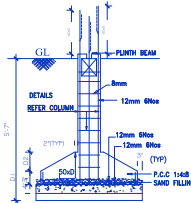
FOUNDATION DETAILS SCALE : 1:50.
