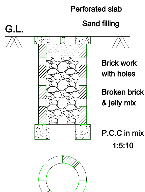
PERCOLATION PIT (NOT FOR SCALE)
