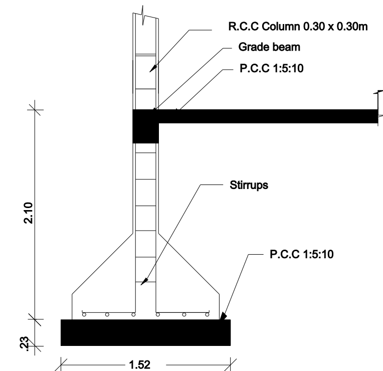
Column Detail
