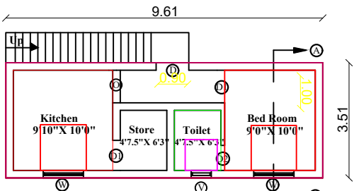
PRO.FIRST FLOOR PLAN
