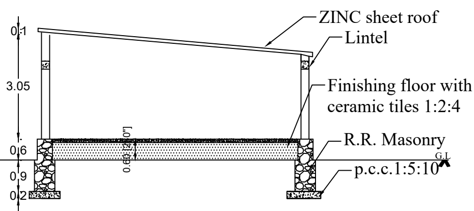
SECTION AB
