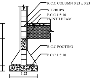
COLUMN DETAILS
