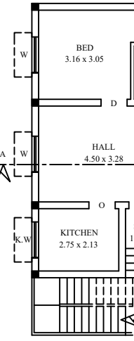
GROUND FLOOR
