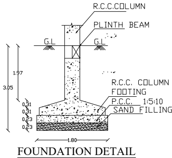
FOUNDATION DETAIL
