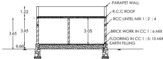
SECTION ON AB & ( HALF ELEVATION)
