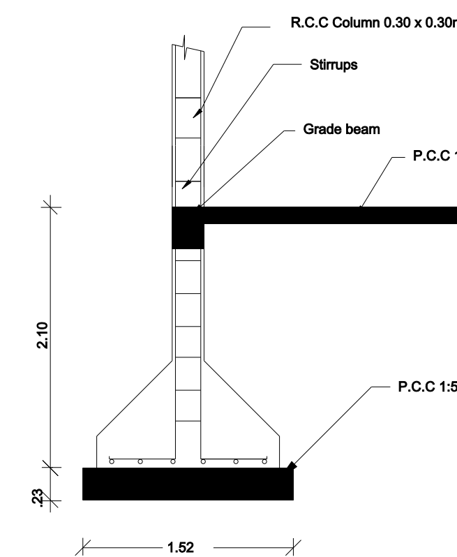
Column Detail
