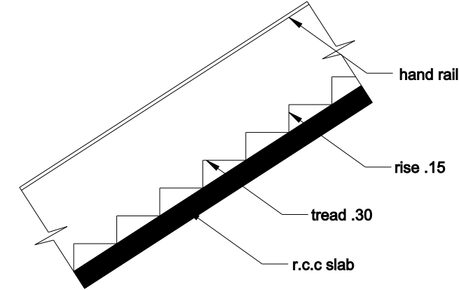
Stair
