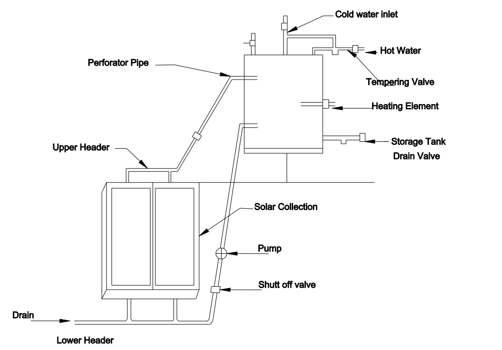
Details Of Solar Water Heater (NTS)
