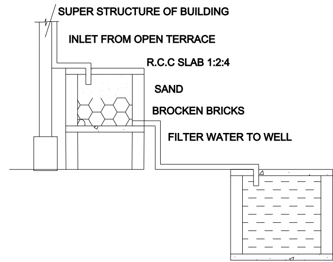
Rainwater harvesting
