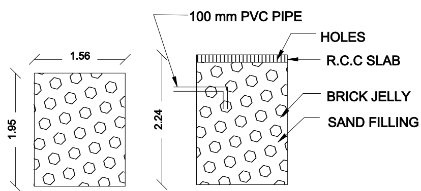
PLAN & SECTION OF RAINWATER COLLECTION TANK
