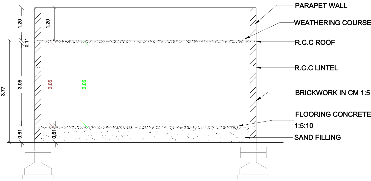
SECTION
