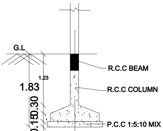
SECTION OF FOOTING
